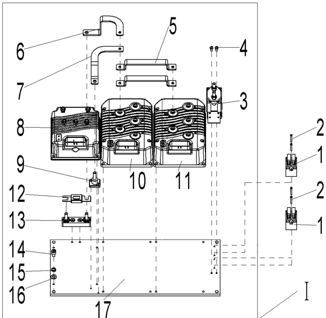
Fig. 27 Electric controller components
