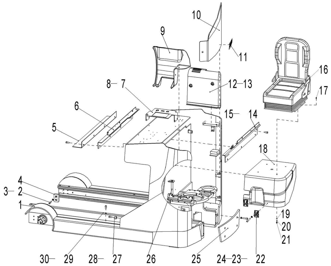
Fig. 11 Truck body
