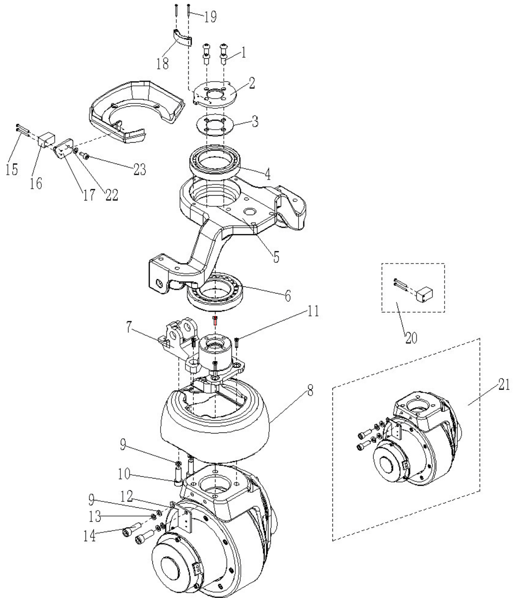
Fig. 4 Driving unit
