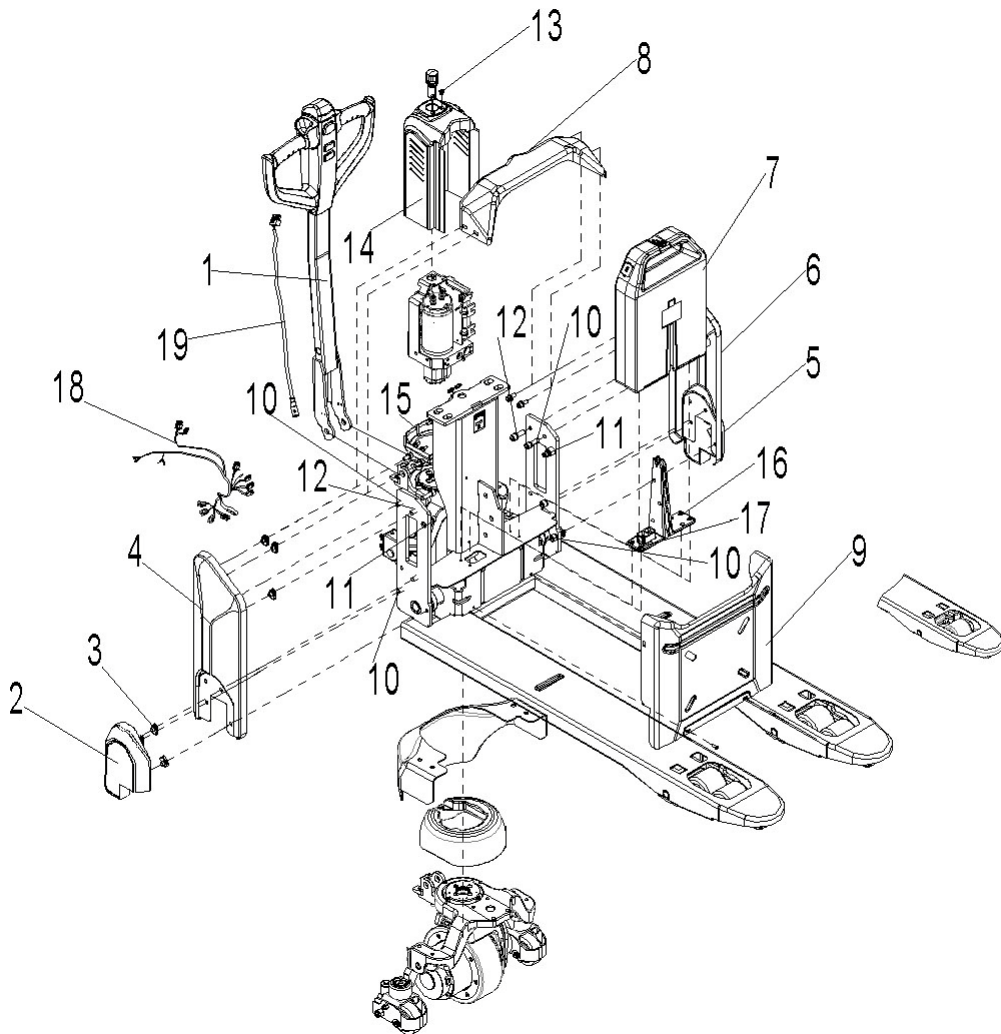
Fig. 13 Truck Components
