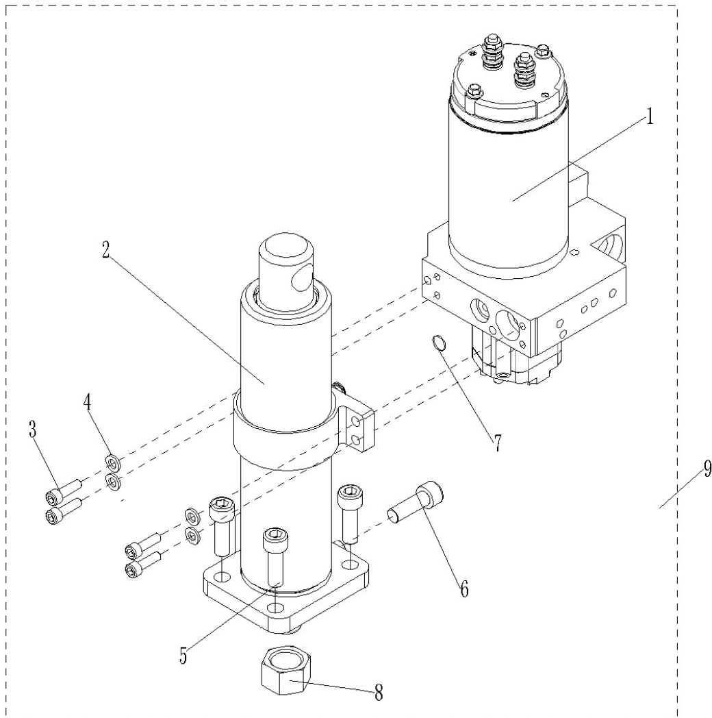
Fig. 8 Hydraulic Components
