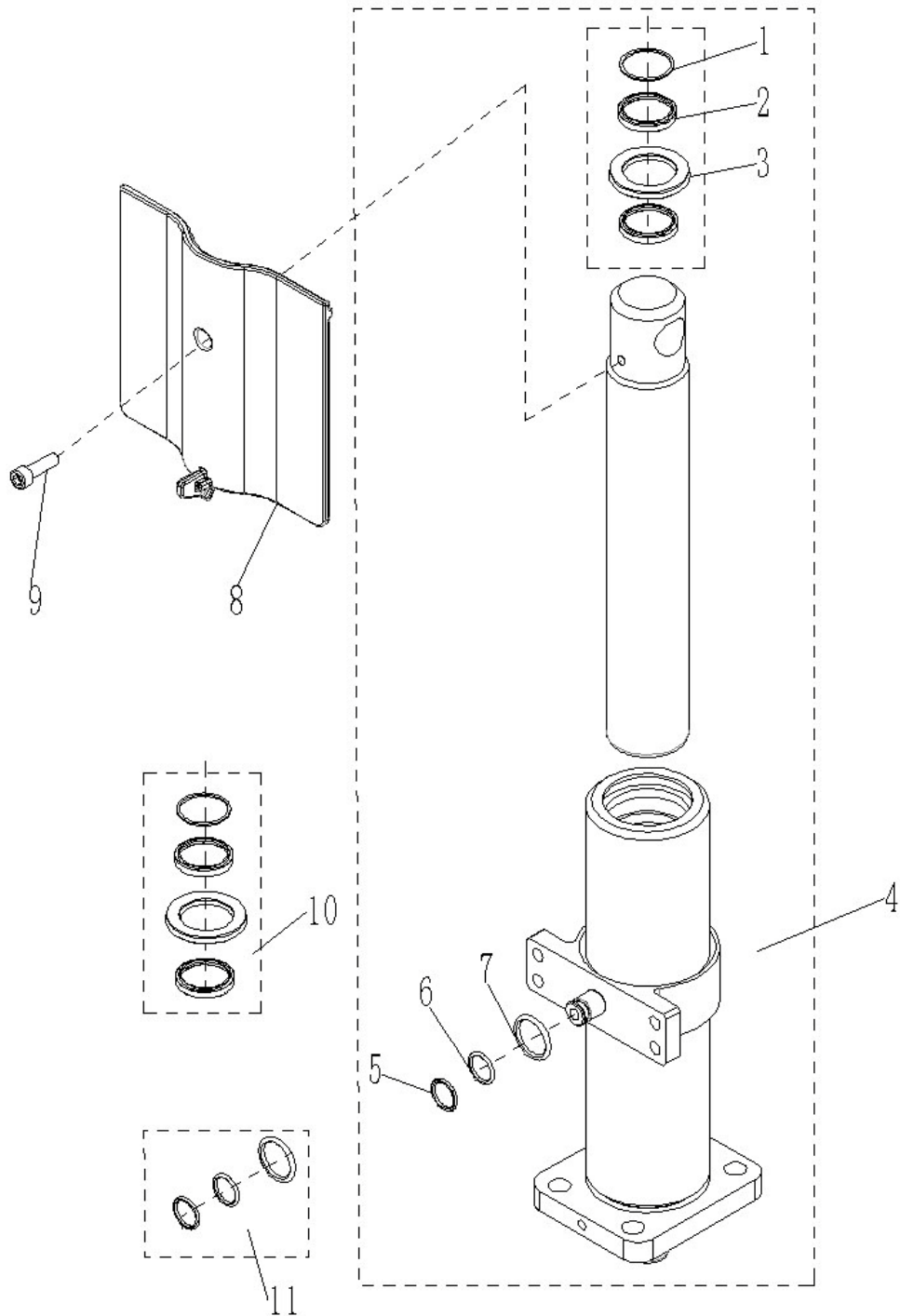
Fig. 6 Cylinder
