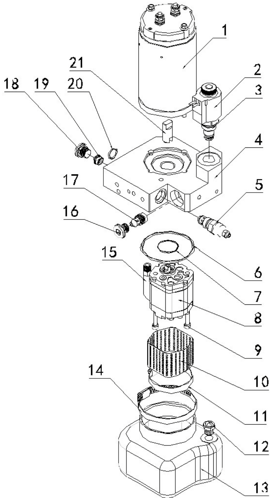
Fig. 7 Power unit
